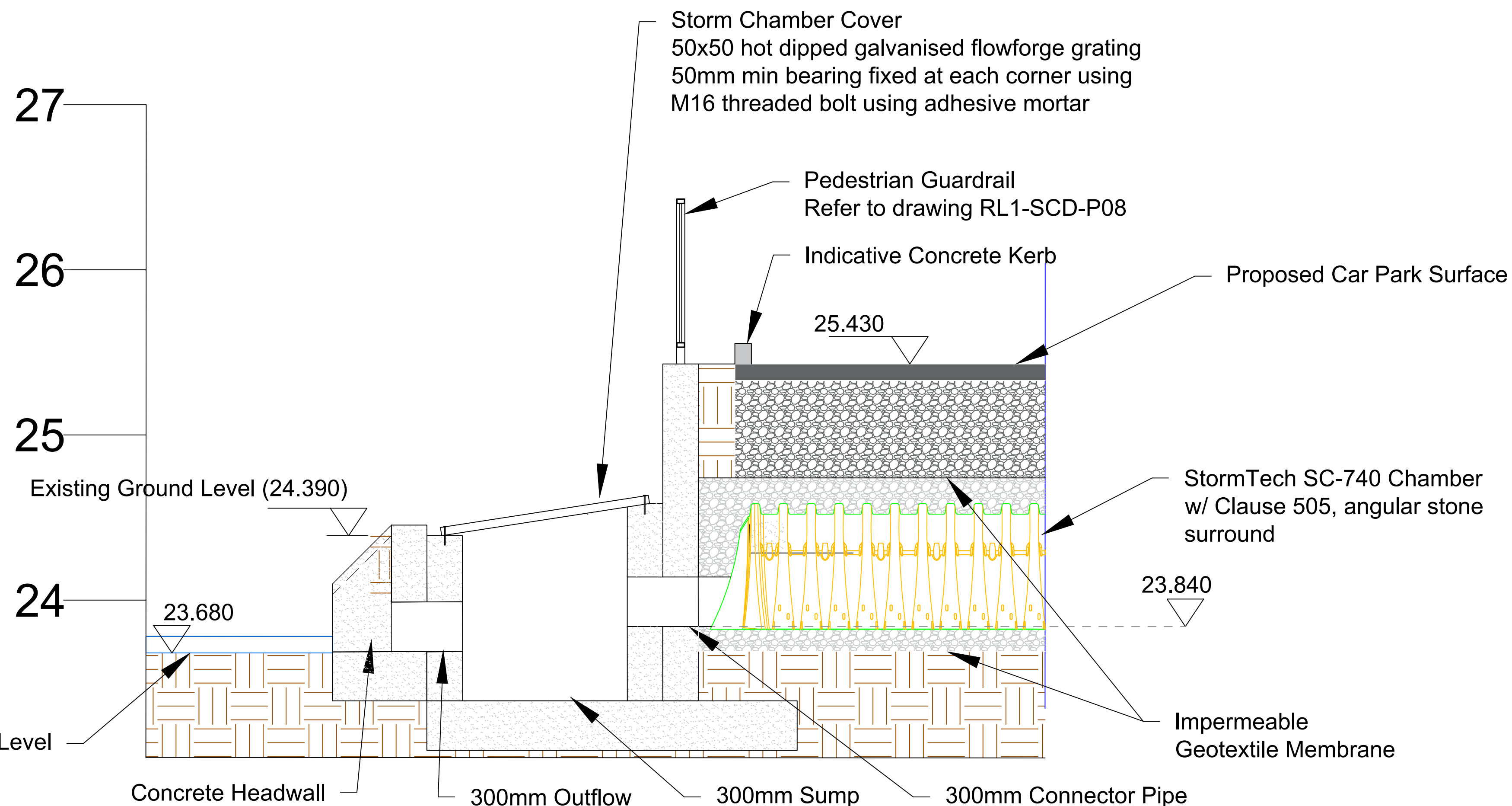
Section C-C
